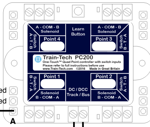
Control using a Train-Tech Mimic switch NB Mimic Lights can be used to indicate point position
