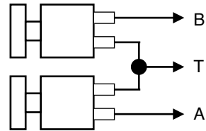
2 Push buttons (momentary)
