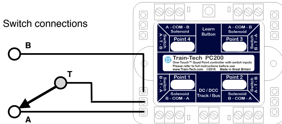
3 Position centre sprung Toggle switch (momentary)
